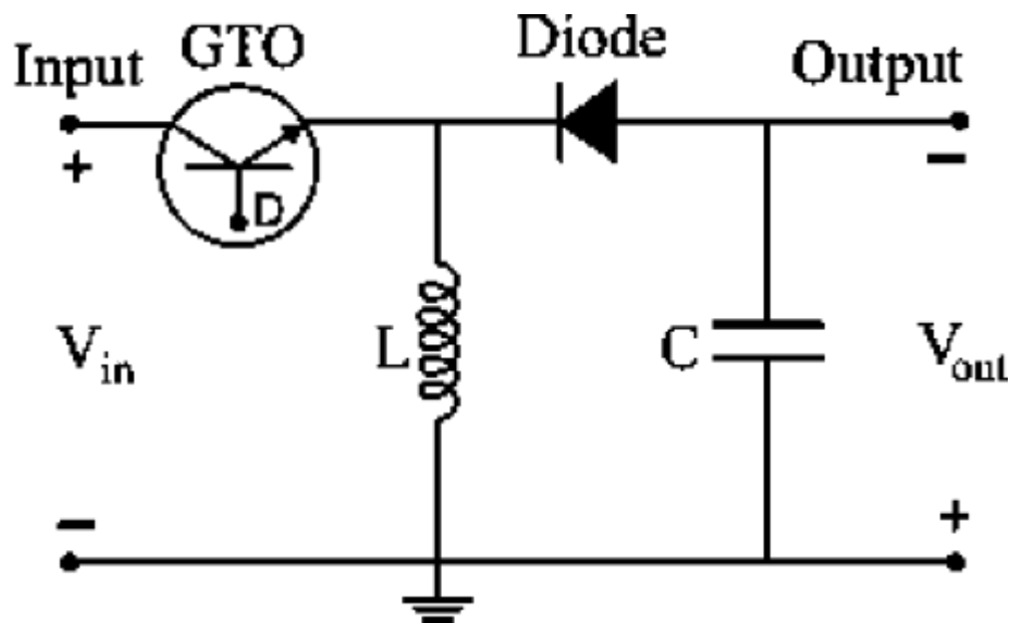
FIGURE 3. Buck-boost topology.
