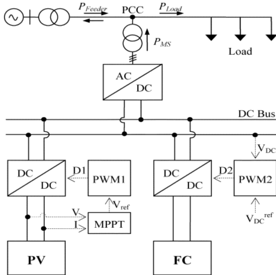
FIGURE 1. Grid-connected PV-FC hybrid system
