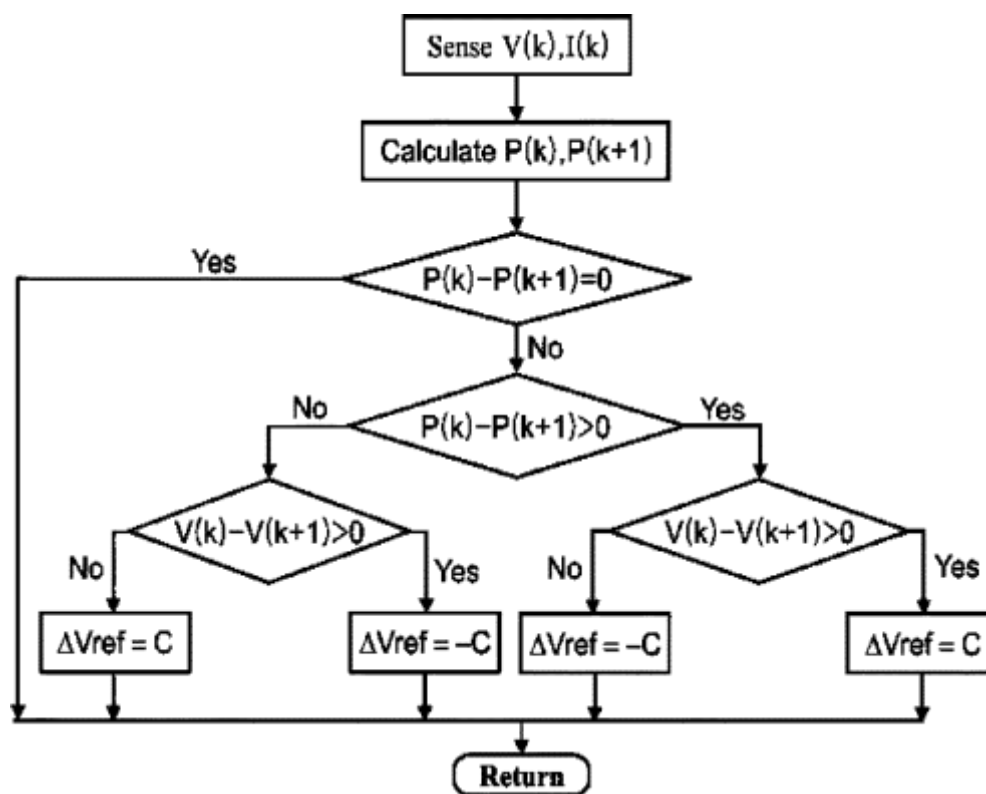
FIGURE 2. P&amp;O MPPT algorithm.
