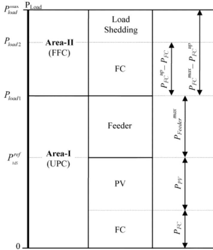
FIGURE 4. Overall operating strategy for the grid-connected hybrid system
