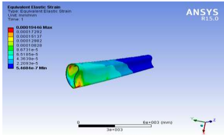
FIGURE 7. Strain in S-glass epoxy 30 0 twist blade angle
