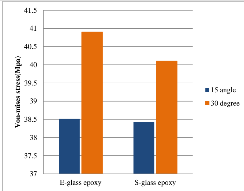
FIGURE 8. Von-mises Stress of Different Materials in Mpa
