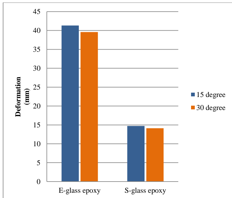
FIGURE 9. Deformation in Different Materials in mm
