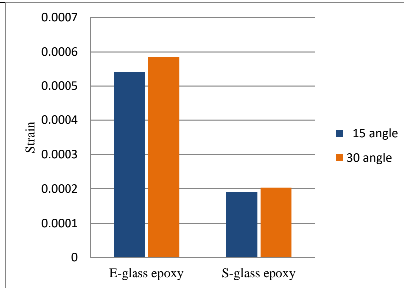
FIGURE 10. Strain in Different Materials
