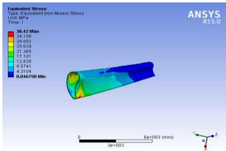
FIGURE 5. Von-misses stress in S-glass epoxy 15 0 twist blade angle
