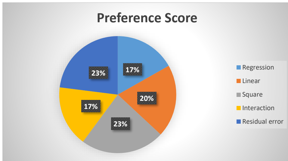
FIGURE 3. Preference Score
