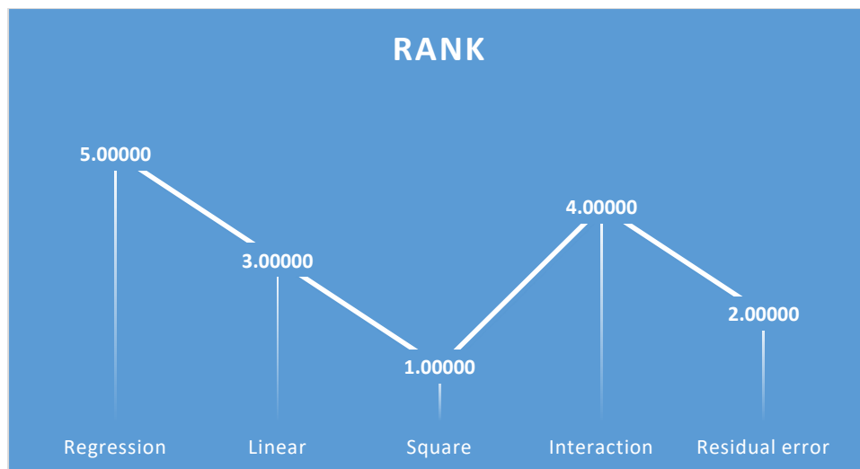
FIGURE 4. Rank
