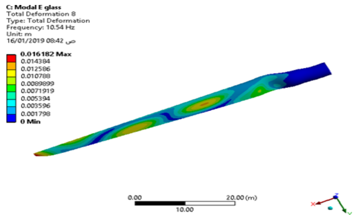
FIGURE 15. 2nd mode shape of E-glass fiber blade
