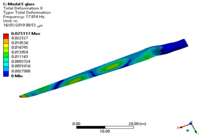
FIGURE 18. 2nd mode shape of Kevlar blade
