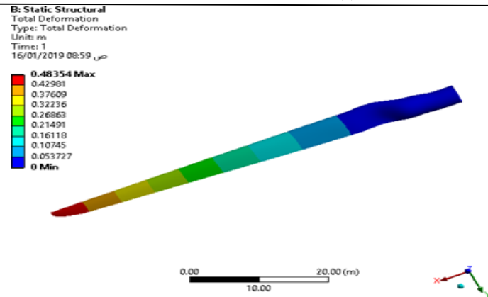
FIGURE 12. Total deformation of CFRP, rated speed
