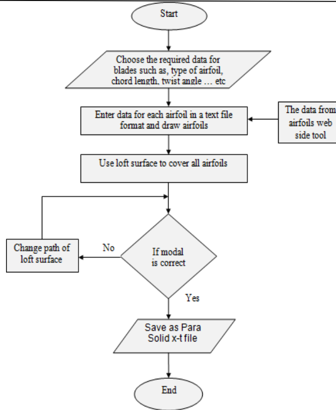
FIGURE 3. Flowchart of the process to build 3D model of the wind turbine blade
