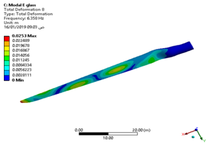
FIGURE 21. 2nd mode shape of CFRP blade
