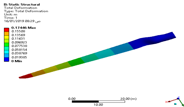
FIGURE 8. Total deformation of E-glass fiber, rated speed
