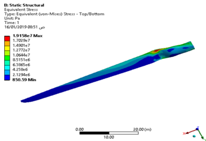
FIGURE 11. Von-Mises stress of Kevlar, rated speed
