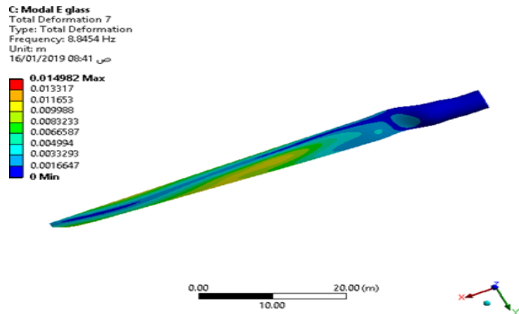
FIGURE 14. 1st mode shape of E-glass fiber blade
