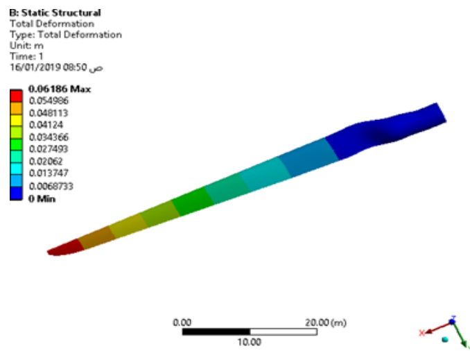
FIGURE 10. Total deformation of Kevlar, rated speed
