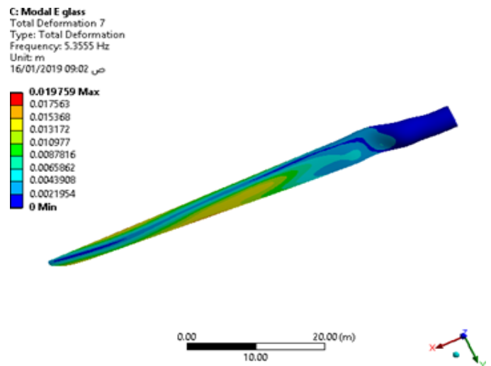
FIGURE 20. 1st mode shape of CFRP blade
