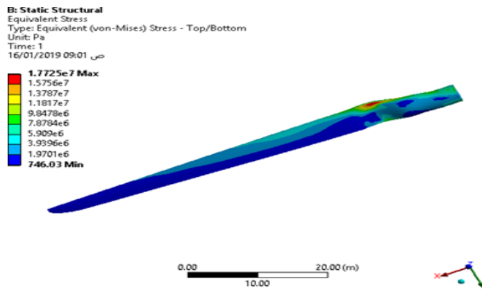
FIGURE 13. Von-Mises stress of CFRP, rated speed
