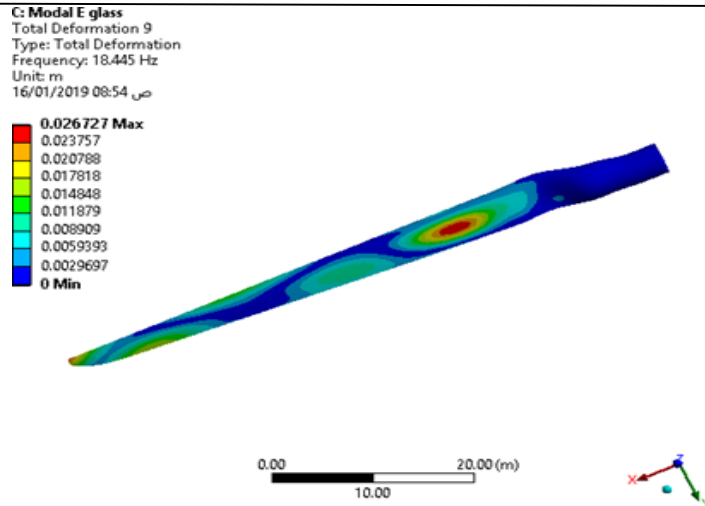
FIGURE 19. 3rd mode shape of Kevlar blade
