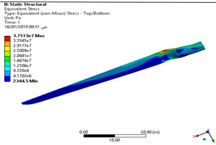
FIGURE 9. Von-Mises stress of E-glass fiber, rated speed
