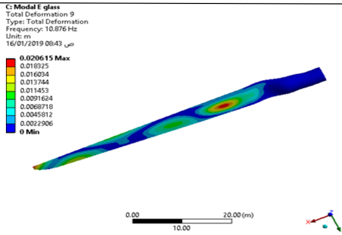
FIGURE 16. 3rd mode shape of E-glass fiber blade
