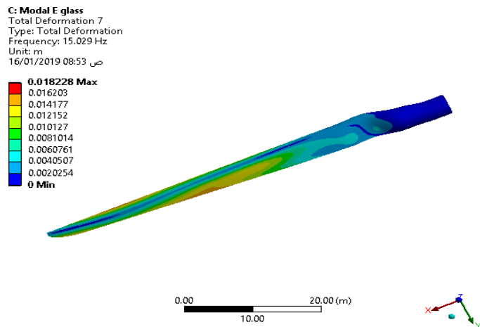
FIGURE 17. 1st mode shape of kevlar blade
