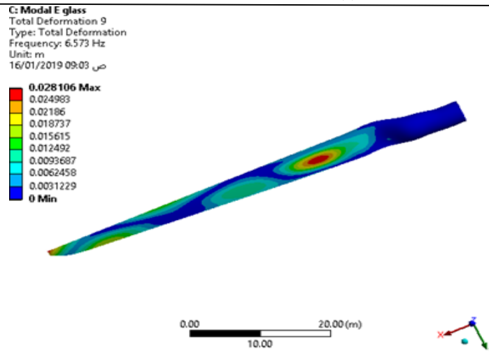
FIGURE 22. 3rd mode shape of CFRP blade
