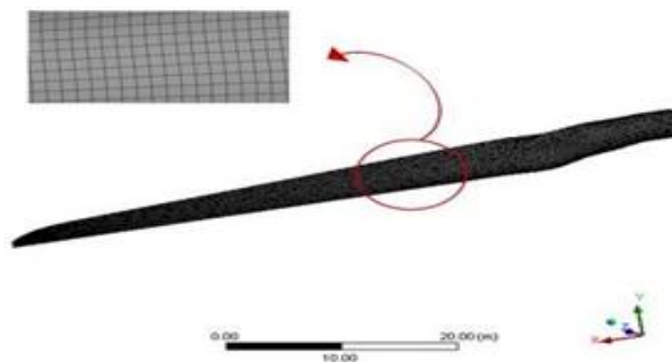
FIGURE 7. Finite element model of 5-MW turbine blade
