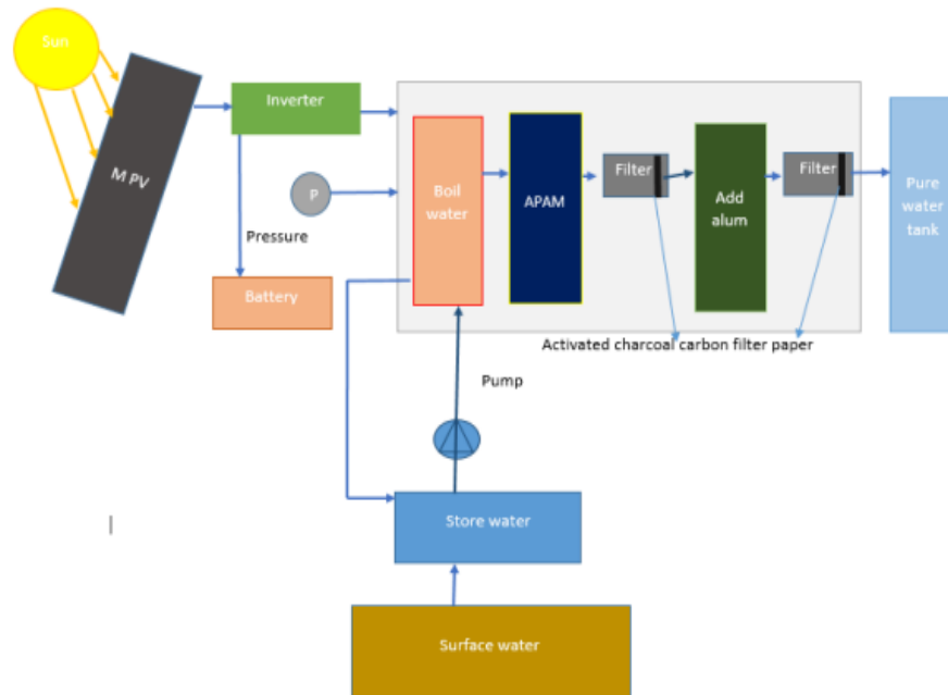
FIGURE 1. Solar Based Water Purification Process
