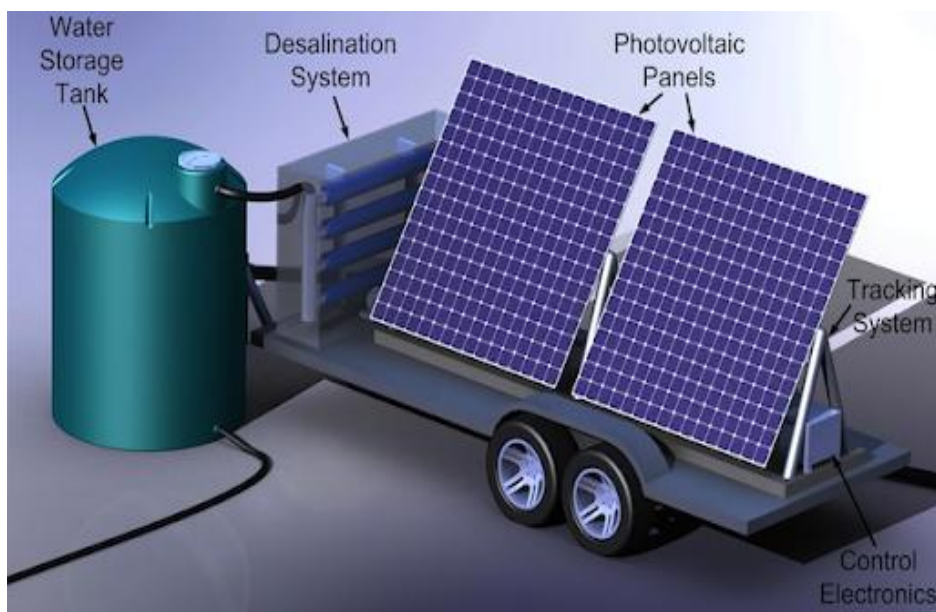
FIGURE 3. Solar Based RO Plant
