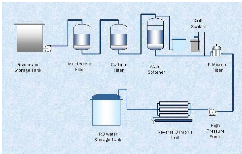
FIGURE 2. Reverse osmosis water purification plant
