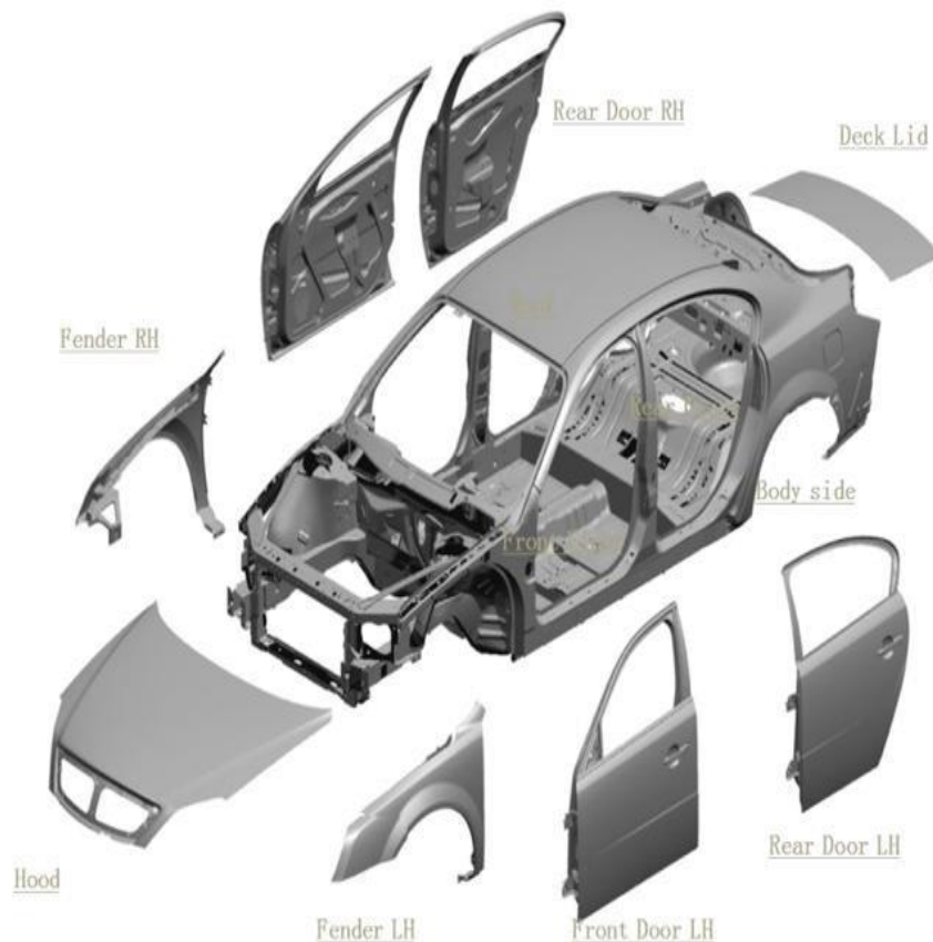
FIGURE 2. Sheet Metal Panels for Car Body ()
