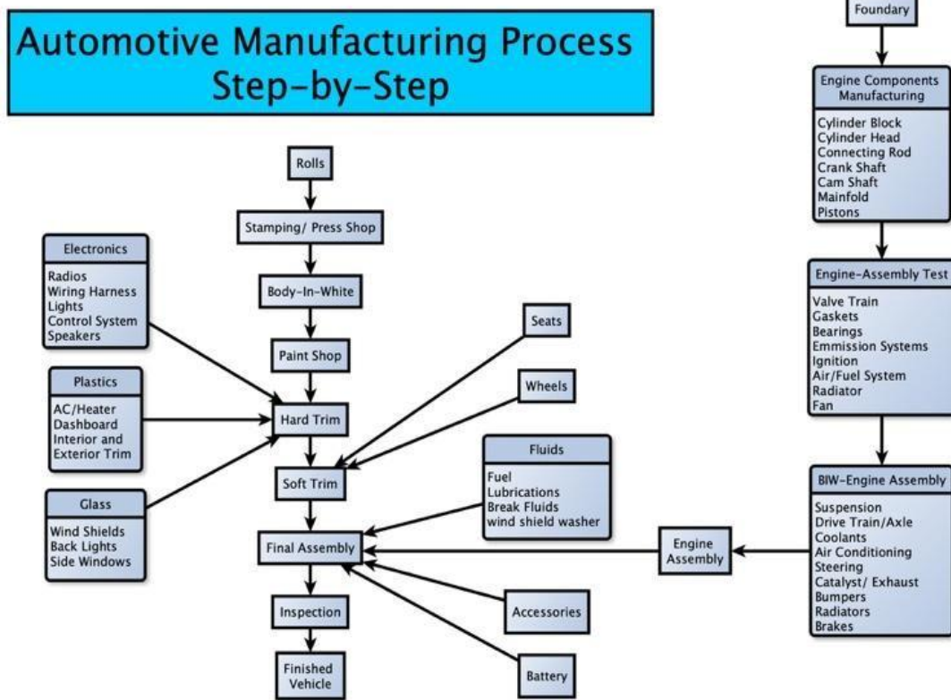
FIGURE 1. Major Departments and workflow for Automotive Plant (2)
