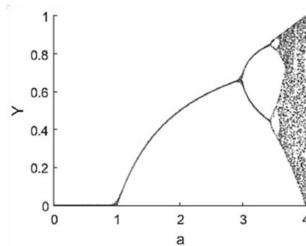
FIGURE 3. Bifurcation Diagram of the Logistic Map
