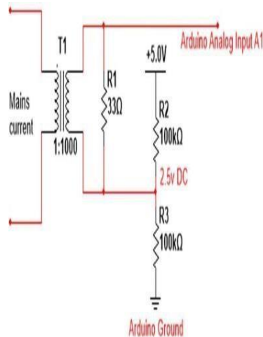
FIGURE 10. Circuit Diagram
