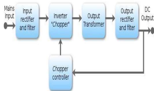
FIGURE 3. Block Diagram of SMPS
