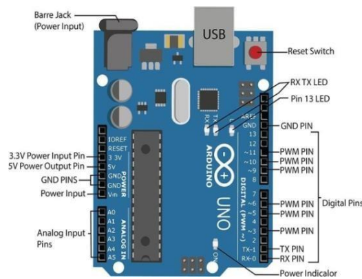
FIGURE 5. Pin Diagram
