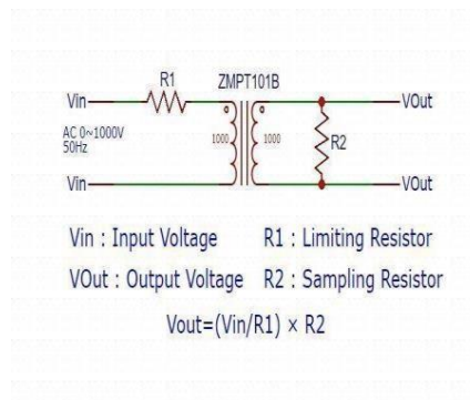
FIGURE 8. Zmpt101b Wiring Diagram
