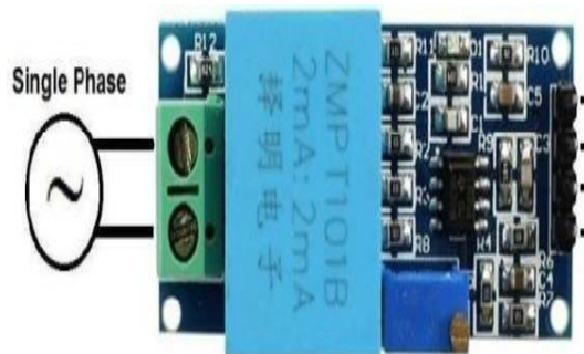
FIGURE 7. Voltage sensor
