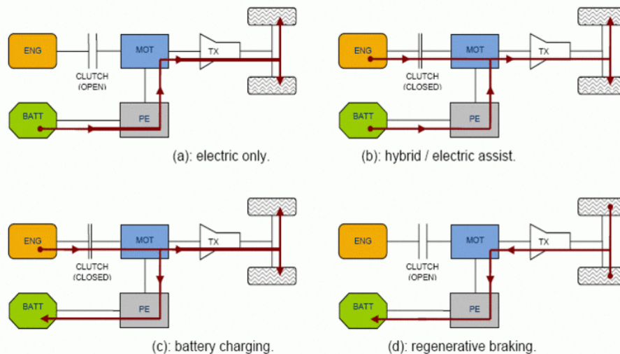
FIGURE 1. Working Principle of Hybrid Vehicle
