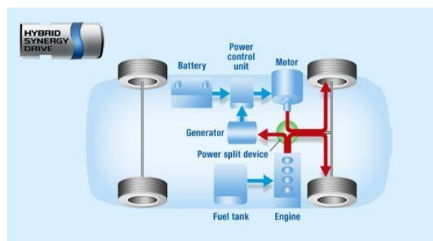
Figure 8. Diagram of Toyota Hybrid System
