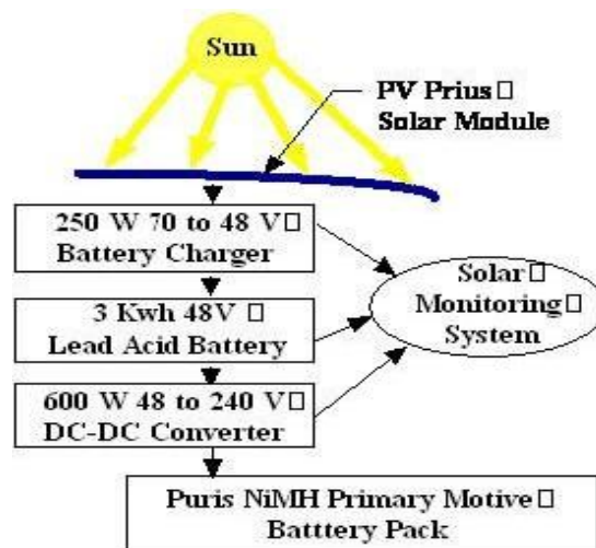
Figure 11. Connection Diagram for Solar Components of the Photovoltaic (PV) Prius
