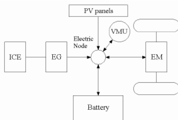
FIGURE 7. Basic Diagram of series Hybrid Solar Vehicle [6]
