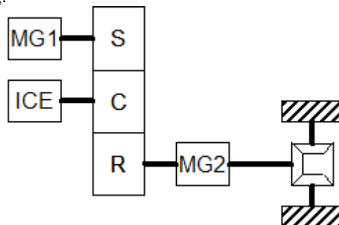
FIGURE 9. Hybrid Synergy Drive mechanism
