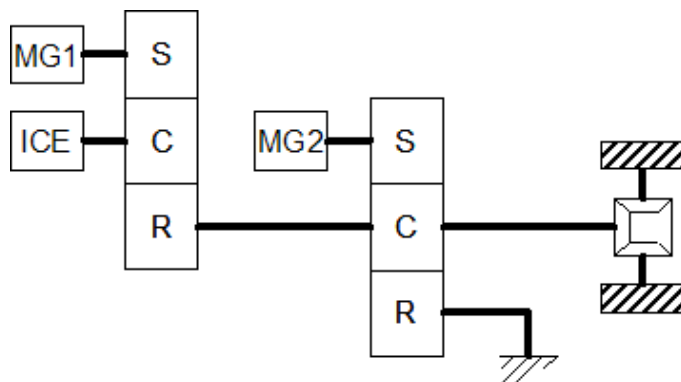
Figure 10. Hybrid Synergy Drive mechanism
