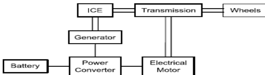
FIGURE 6. Series-Parallel Hybrid Structure
