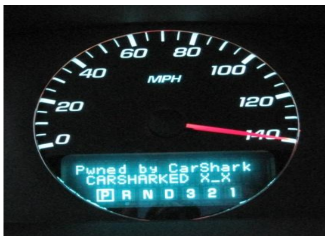
FIGURE 6. Displaying an arbitrary message and a false speedometer reading on the Driver Information Center. Note that the car is in Park.
