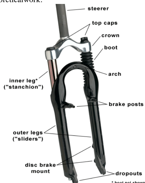
FIGURE 2. Front suspension
