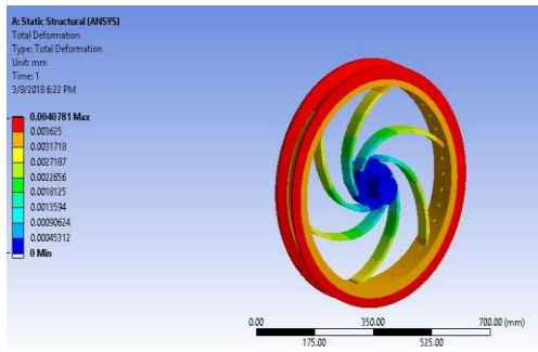
FIGURE8. Deformation FIGURE9. Strain
