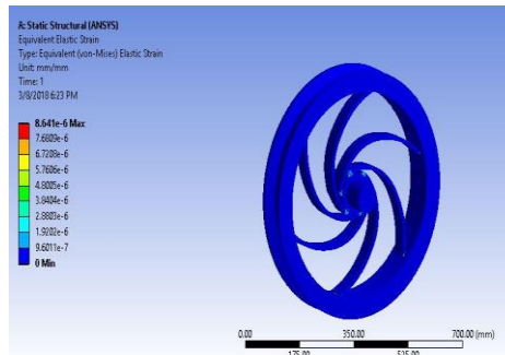
FIGURE8. Deformation FIGURE9. Strain
