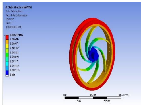
FIGURE 10.DEFORMATION FIGURE 11. Strain
