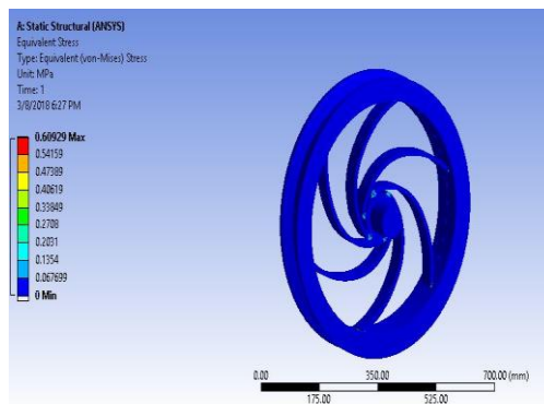
FIGURE 12. Stress
