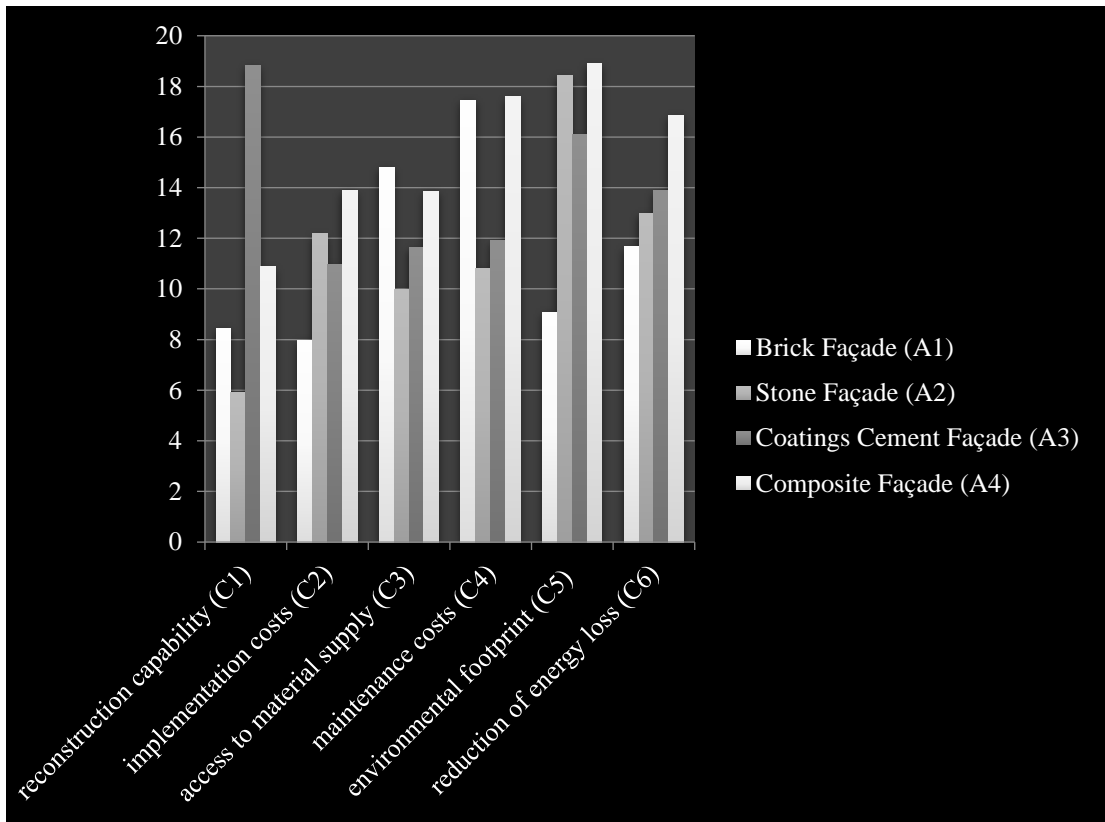
FIGURE 1. Data set for Blast Resistant Buildings
