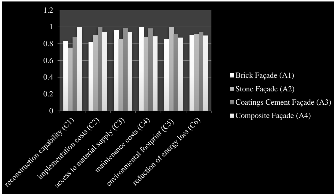
FIGURE 3. Weighted normalized decision matrix
