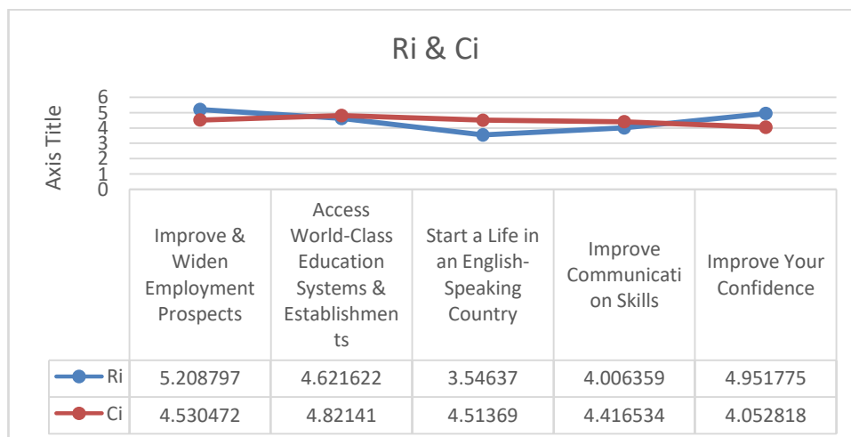
FIGURE 4. Ri & Ci
