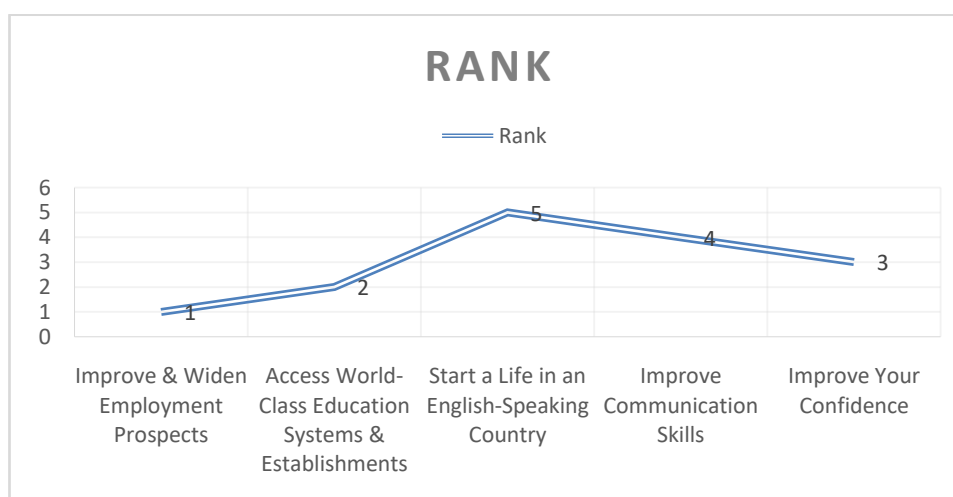
FIGURE 5. Rank
