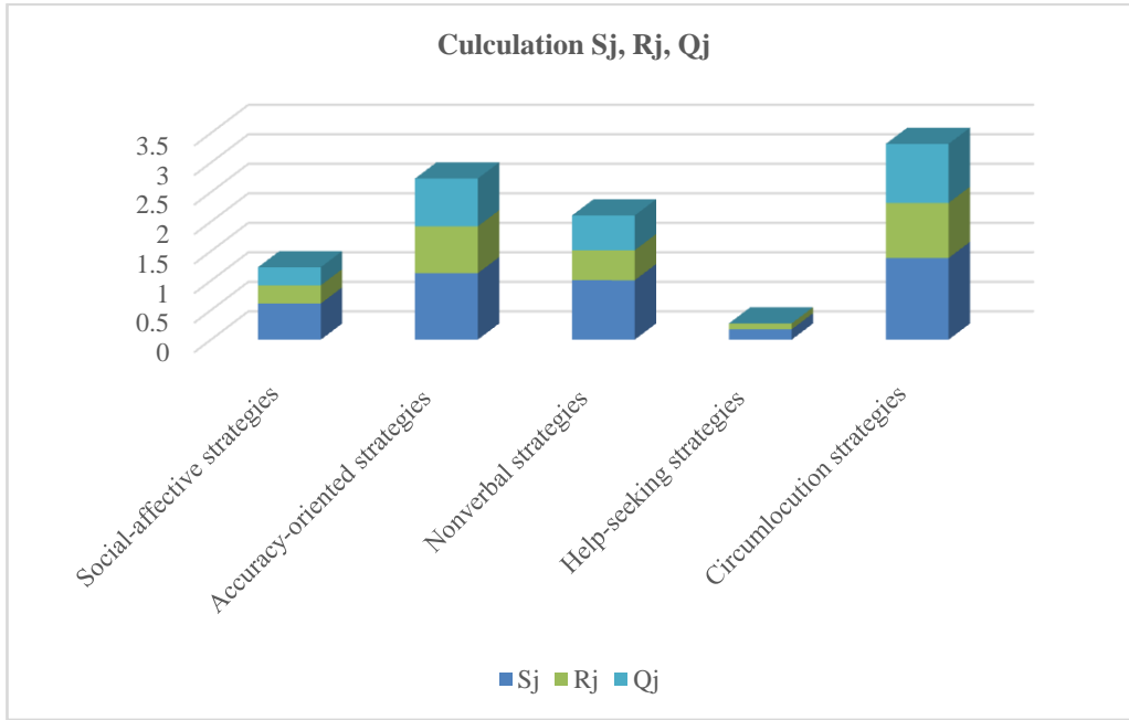
FIGURE 2. Calculation Sj, Rj and Qj
