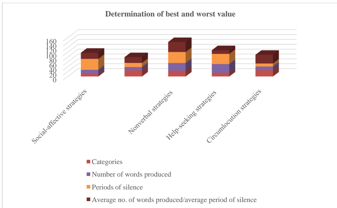
FIGURE 1. Determination of best and worst value of English Communication Development
