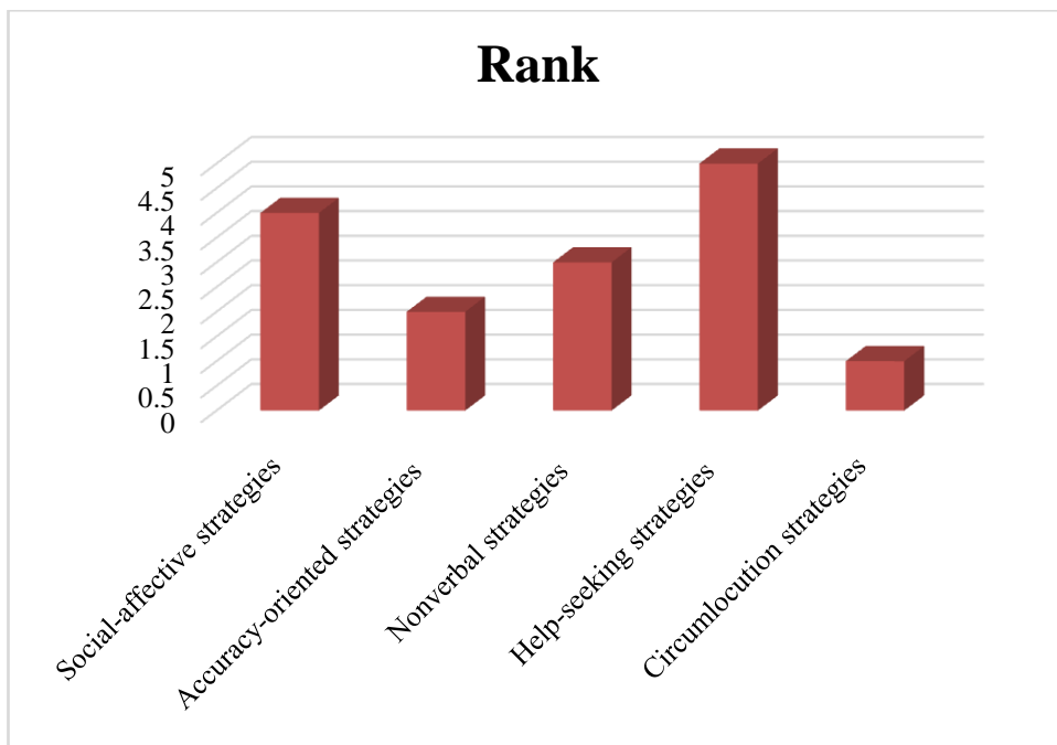
FIGURE 3. Shown the Rank
