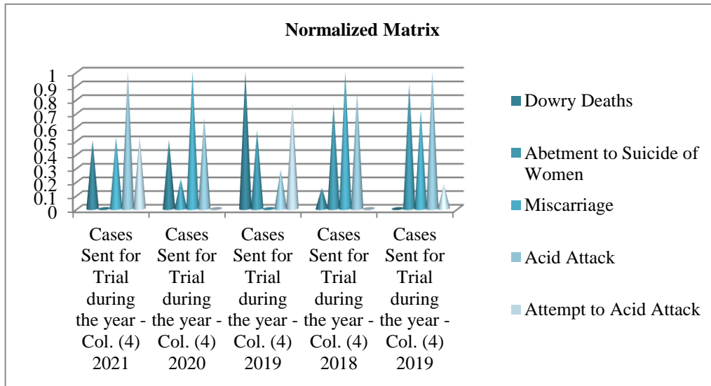
FIGURE 2. Normal matrix
