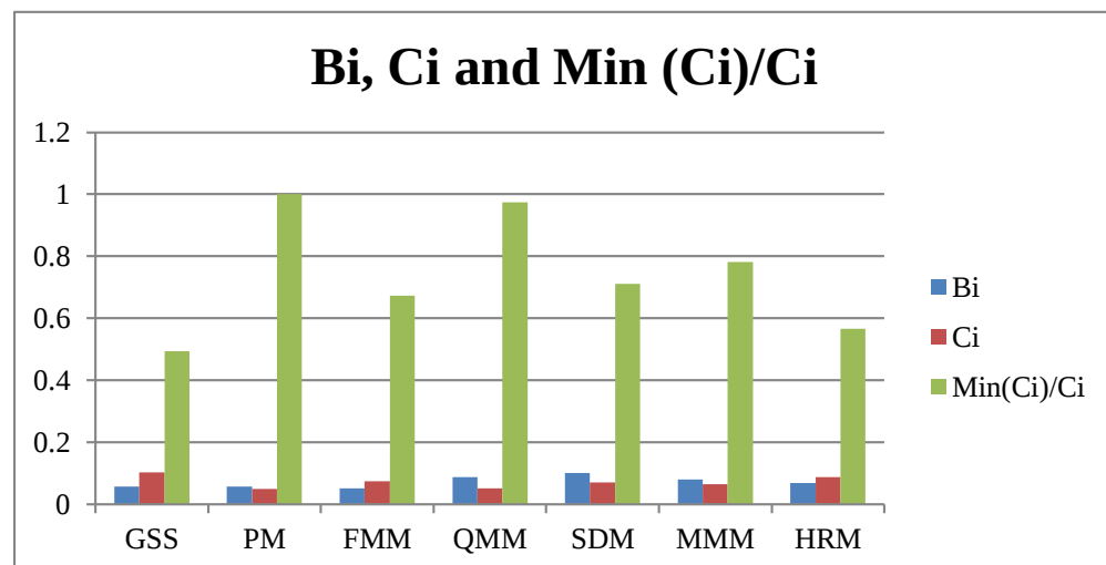
FIGURE 2. Bi, Ci and Min (Ci)/Ci
